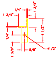
FRAME SECTION VIEW SCALE 1:4
